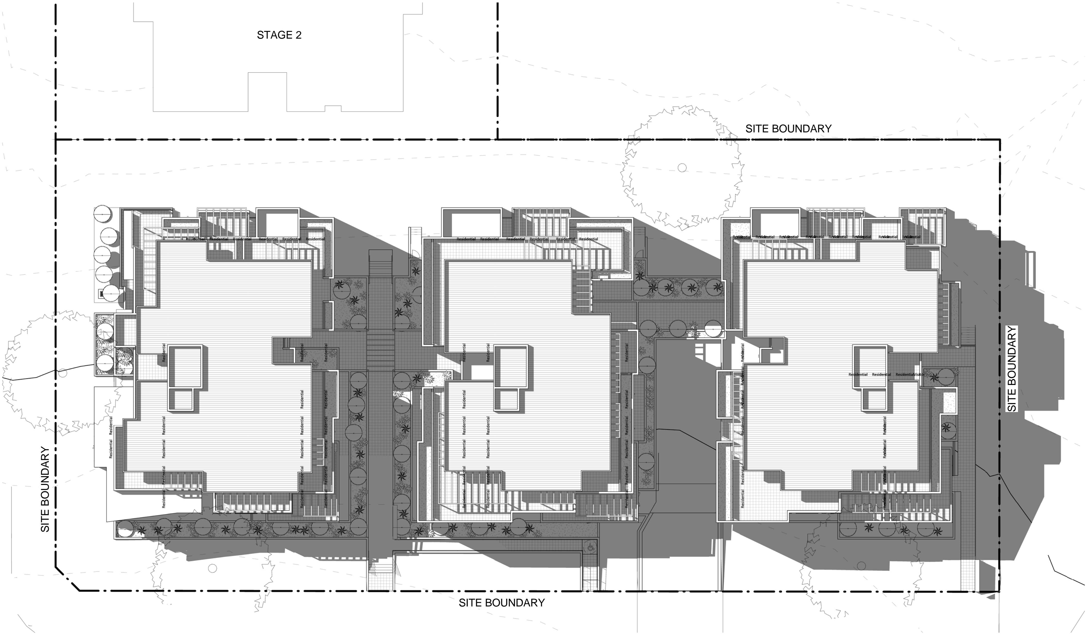
1 3pm SHADOW DIAGRAM - 22nd DECEMBER 1 : 200
